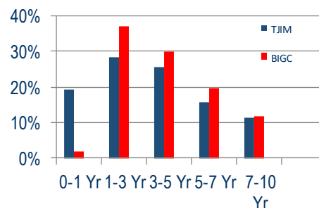
Duration Distribution
