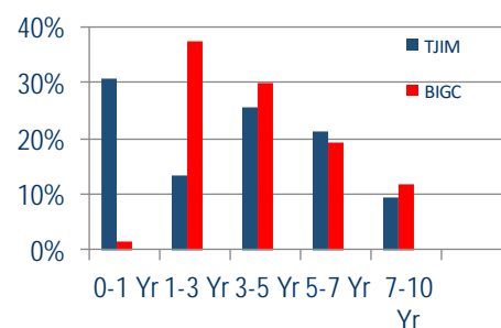
Duration Distribution
